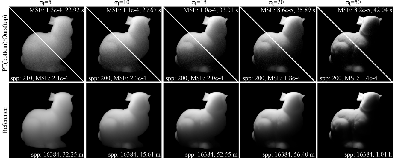
Figure 4. Comparison between our method and volumetric path tracing (equal-time) on media with varying extinction coefficients \sigma_t \in \{5, 10, 15, 20, 50\} . Our method produces better results than path tracing consistently. The sample rate of the source scene is set as 256.
