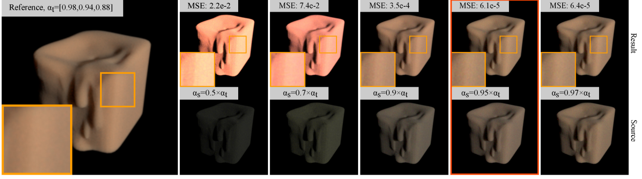
Figure 6. Predicted results (top) from different sources (bottom) on the Candle scene. When the source albedo is far from the target albedo, there is obvious color bias after the prediction.
