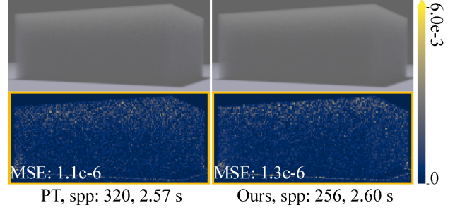
Figure 9. Failure case: comparison between our method and path tracing on rendering the low-albedo media. The source \alpha_s = 0.9 \times \alpha_t and the target \alpha_t = 0.5 .
