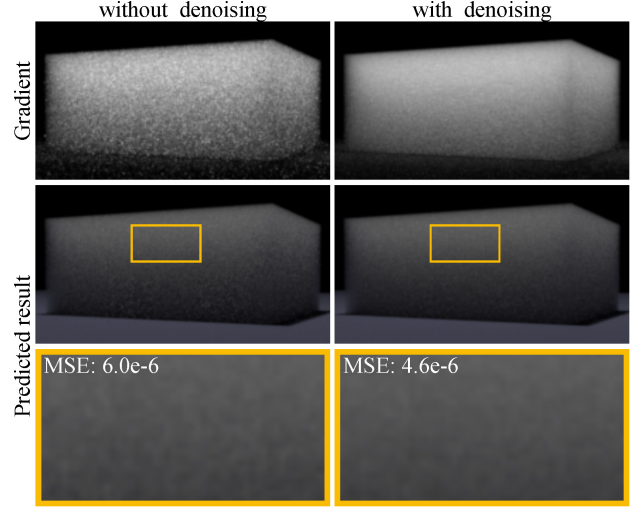
Figure 2. Comparison of gradient images (top) without denoising and with denoising (top) and their predicted results (bottom).
