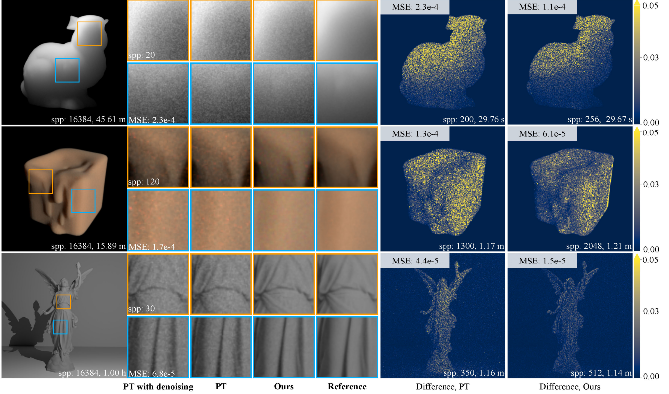
Figure 3. Comparison among our method, temporal denoised path tracing with equal time, path tracing with equal time, and the reference. The difference between path tracing and the reference and the difference between our method and reference are shown in the last two difference maps.
