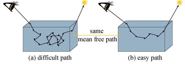
Figure 1. For high-order scattering dominant media, the light path is extremely long, especially when the albedo is high since the attenuation after each scattering is minor; when the albedo is low, the light path will be shortened, since the attenuation becomes quicker. Thus, low-albedo media will have less noise.
