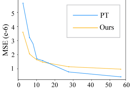
Figure 8. MSE between our method or path tracing with the reference (rendered with 33,768 spp) over varying rendering time on the Cube scene. The error of our method decreases until approximately 16 s and then keeps almost constant. The error before 16 s comes from both variance and bias. After the result is converged, the error comes from bias. Therefore, our method is suitable for rendering with a low time budget.
