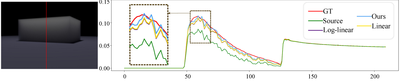
Figure 5. Radiance variation curves on a slice of pixels (the locations are shown as the red line at the left image) of the ground truth (GT), predicted results of linear, log-linear, our prediction functions, and the source image. The source \alpha_s = 0.95 \times \alpha_t and target \alpha_t = 0.95 . Our prediction function is the closest to the ground truth.
