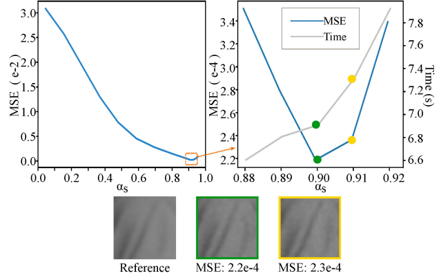
Figure 7. The error (MSE) curve as a function of source albedo \alpha_s on the Lucy scene. The \alpha_s ranges from 0.1 to 0.94 ( 0.1 - 0.97 \times \alpha_t ). The sample rate of the source scene is set as 512. The errors are measured on cropped images ( 30 \times 30 ). The error curve and the time cost curve (rightmost) are on a small range of the source albedo, 0.9 - 0.95 \times \alpha_t . The images corresponding to the orange and green dots are shown at the bottom.
